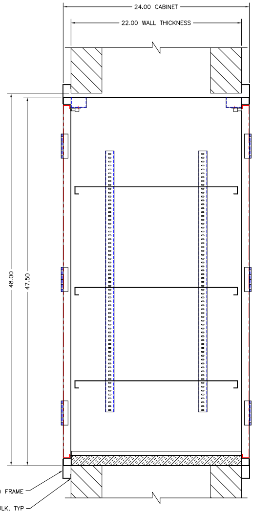
SECTION B-B
